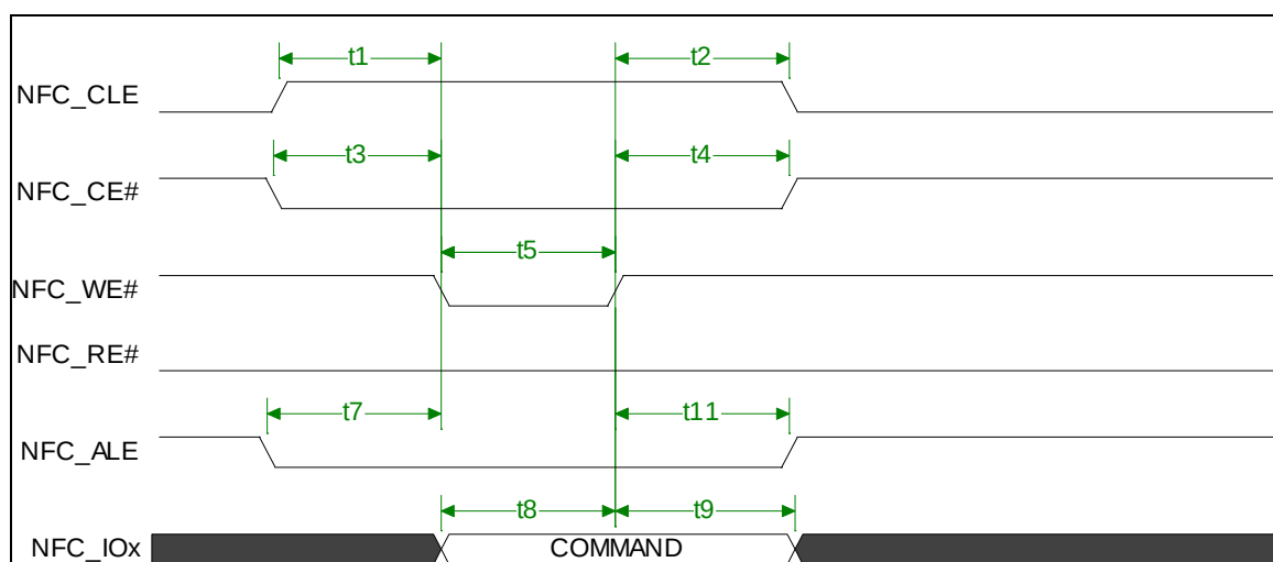
Figure 14-5. Command Latch Cycle
