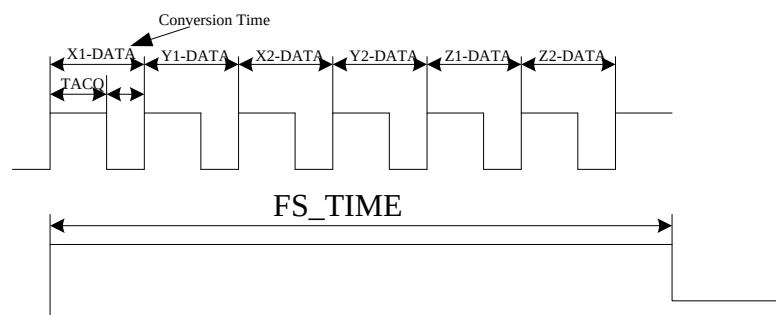
Figure 24-3. Dual Touch And Pressure Measurement
