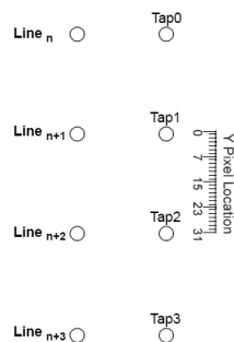
Vertical quantizing
