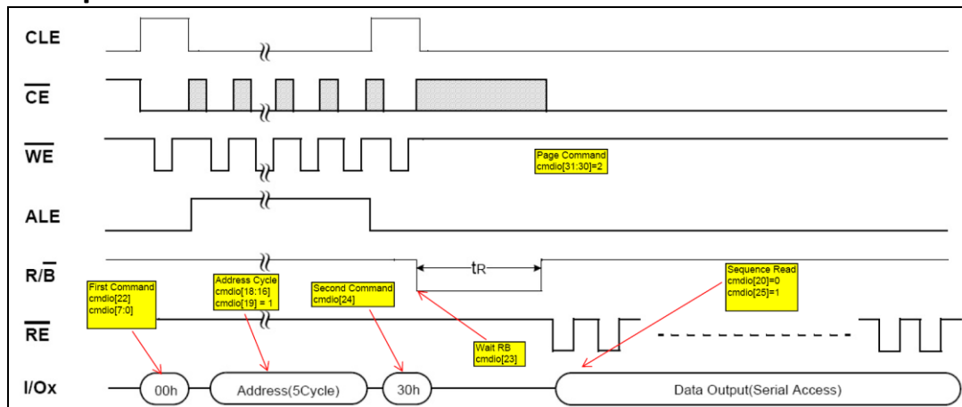
Figure14-12. Page Read Command Diagram
